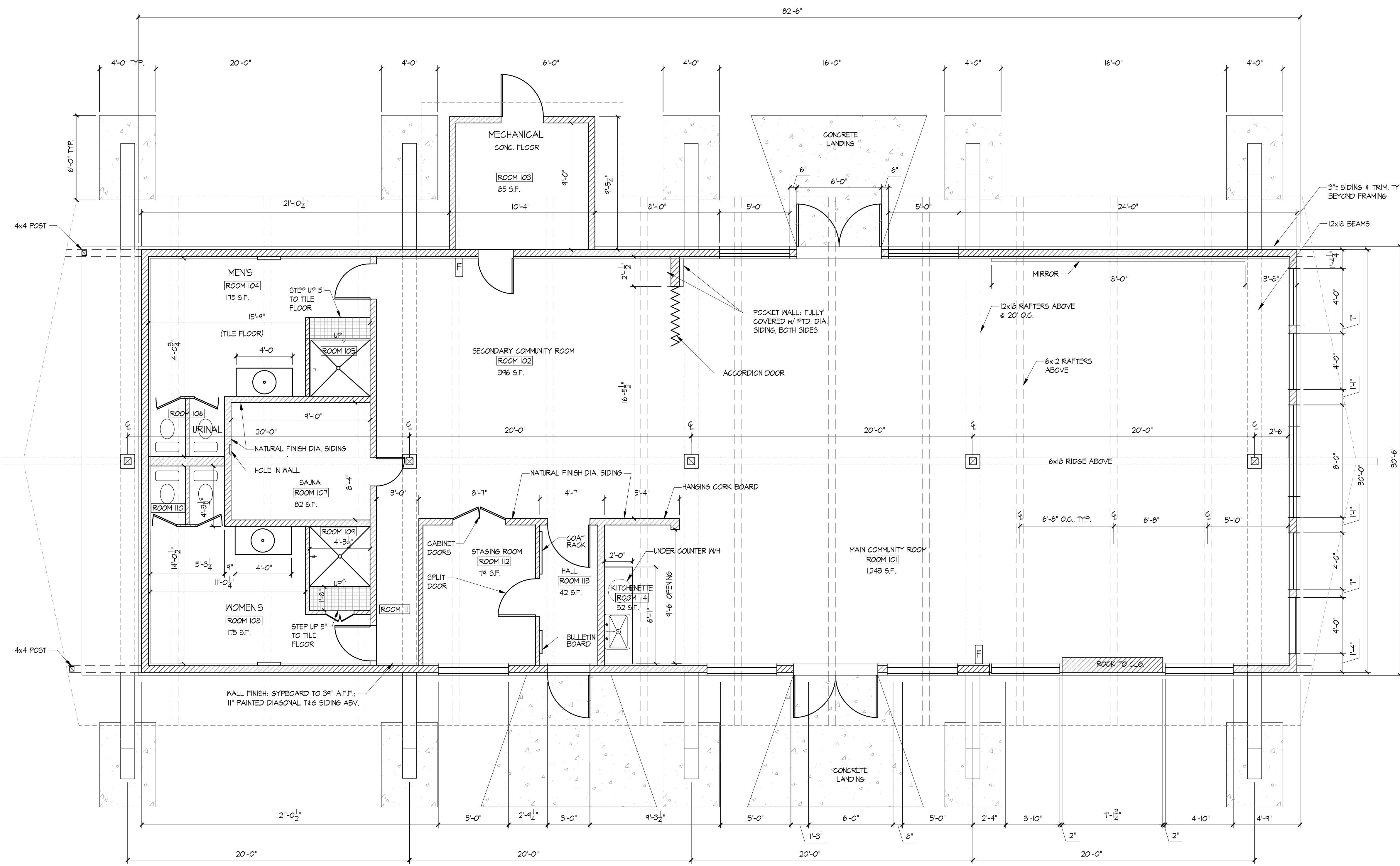
1 FLOOR PLAN 1/4"=1'-0"
